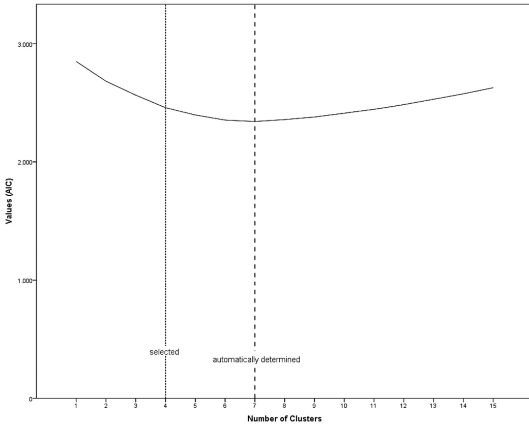
Graph 4: Automatic Clustering (AIC) and number of clusters
